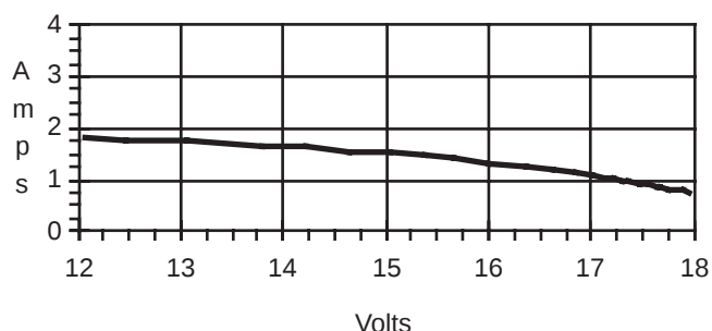
UniSolar UPM880
