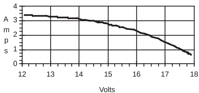
Kyocera LA361K51
