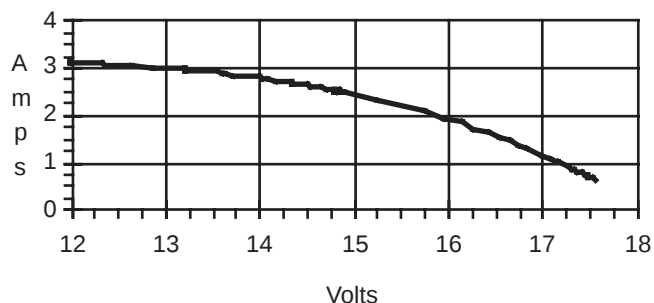
Solec S50
