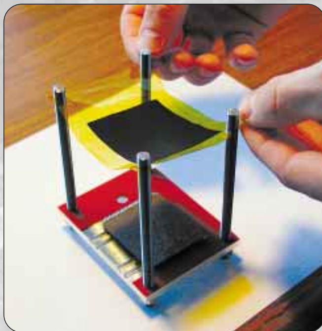
A proton exchange membrane being assembled into the stack of a fuel cell.
