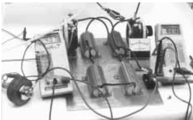
Above: Electrical test system. The four fixed resistors were not used. Photo by Reynaldo Cortez
