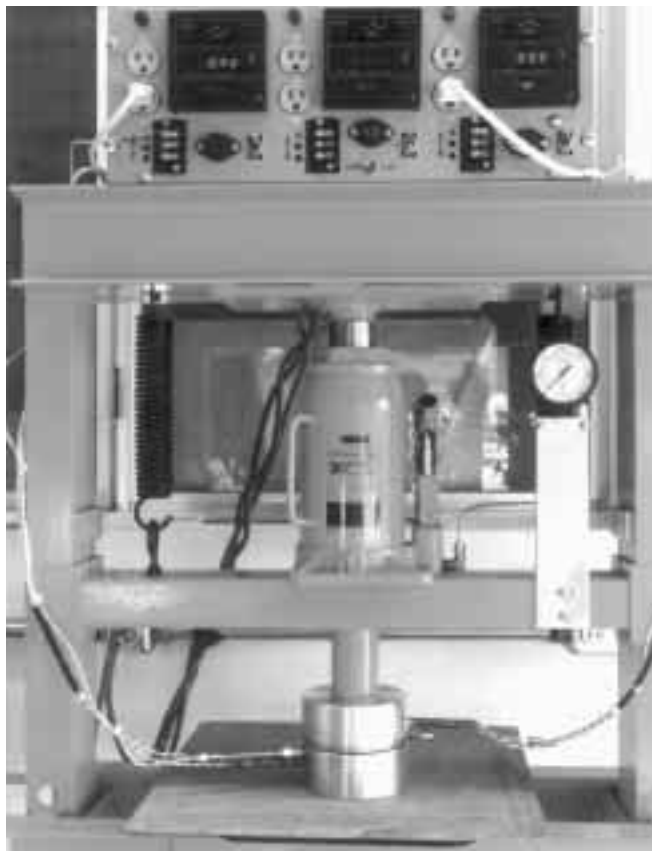
Above: Hot press and heating plates.
