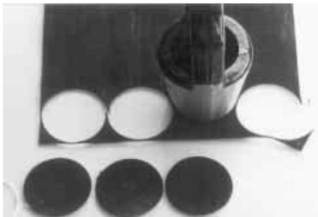
Above: Cutting ELAT catalyst disks.
